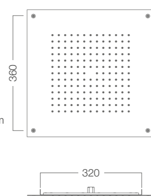
KI 412 ✓ L/H 400 mm ✓ G. 1/2" M
