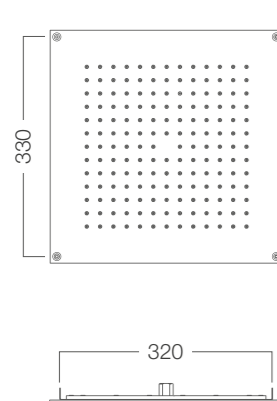
KI 411 ✓ L/H 350 mm ✓ G. 1/2" M
